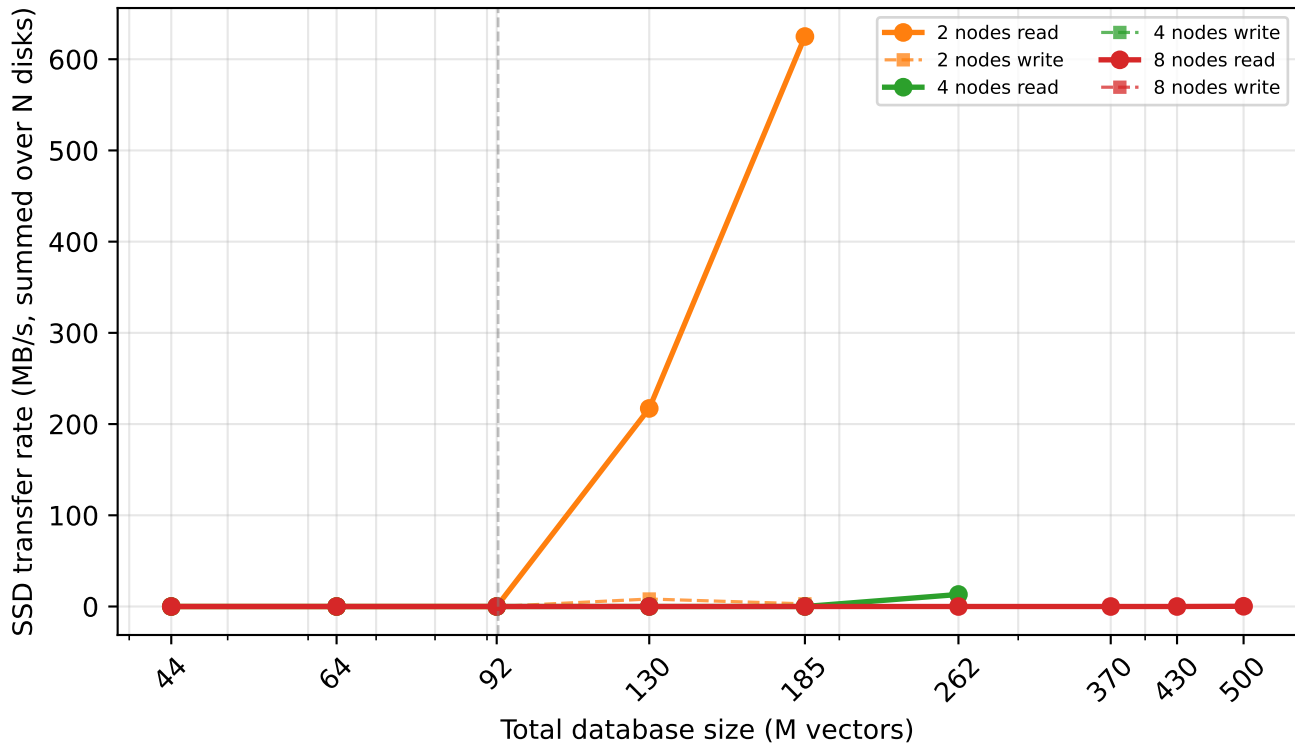
Aggregate SSD transfer rate vs. database size mixed read/write workload, 2/4/8 nodes
