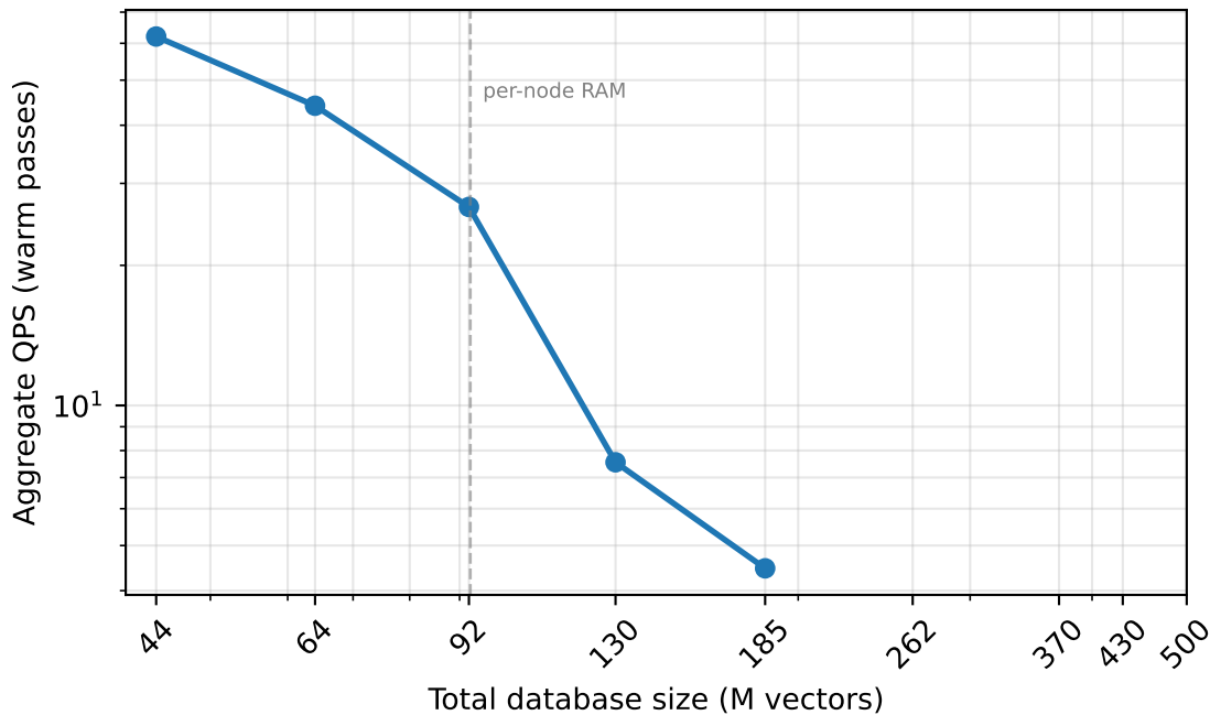
Read-only search throughput vs. database size 1 node
