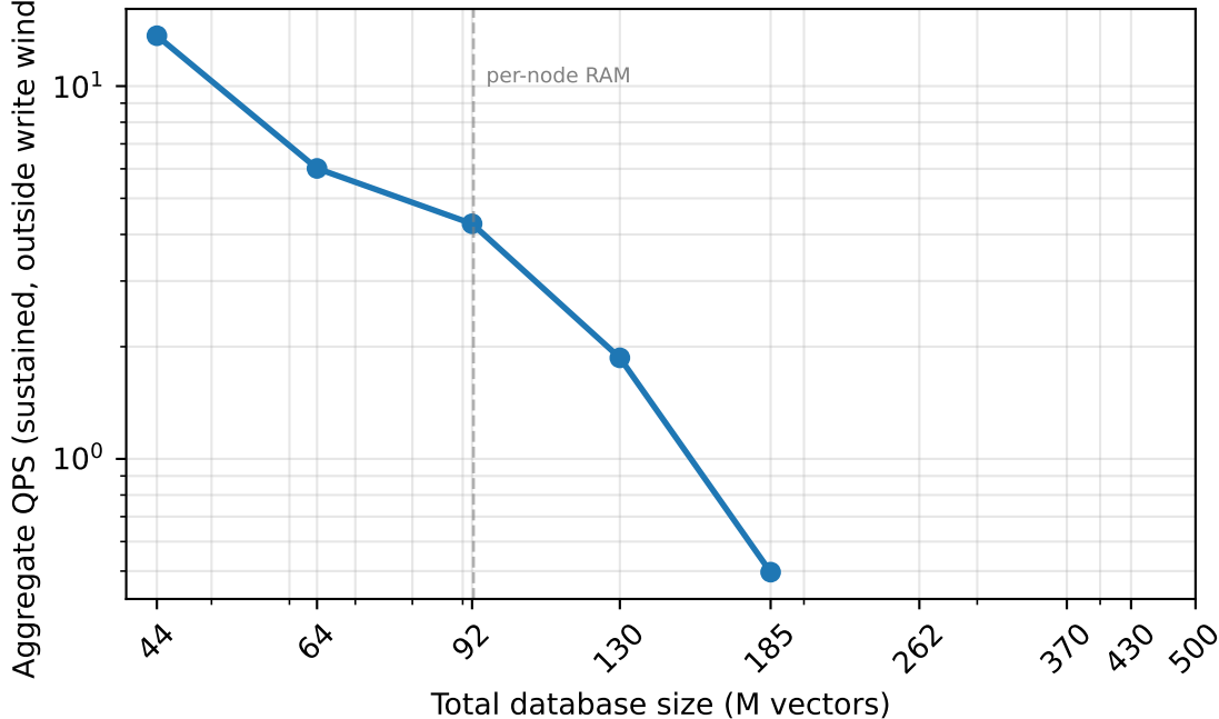
Search throughput under a mixed read/write workload 1 node
