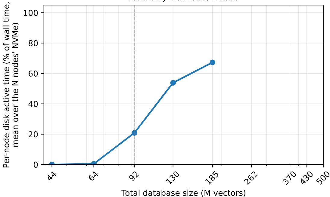
Per-node NVMe active time vs. database size read-only workload, 1 node
