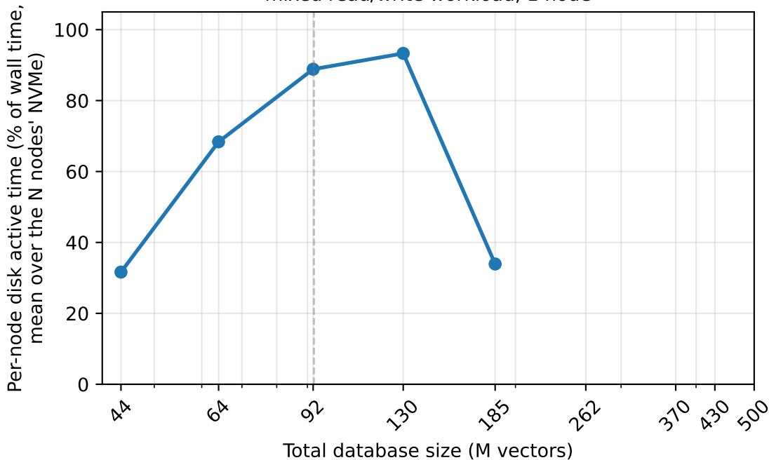
Per-node NVMe active time vs. database size mixed read/write workload, 1 node
