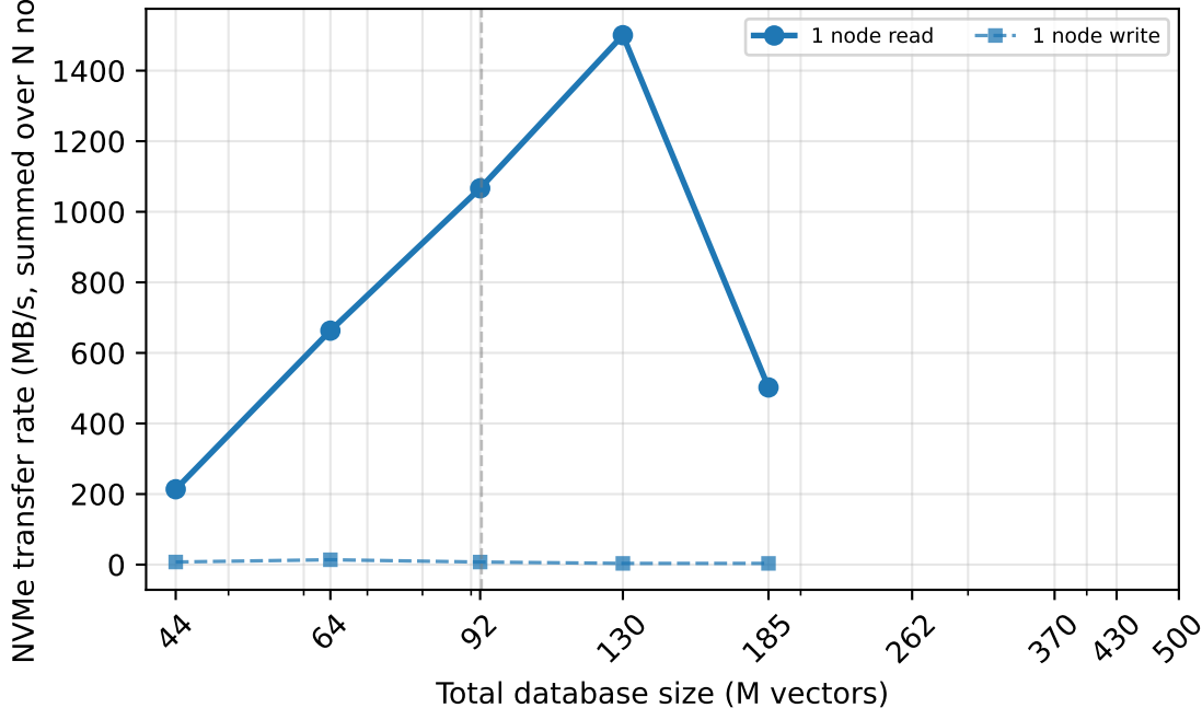
Aggregate NVMe transfer rate vs. database size mixed read/write workload, 1 node
