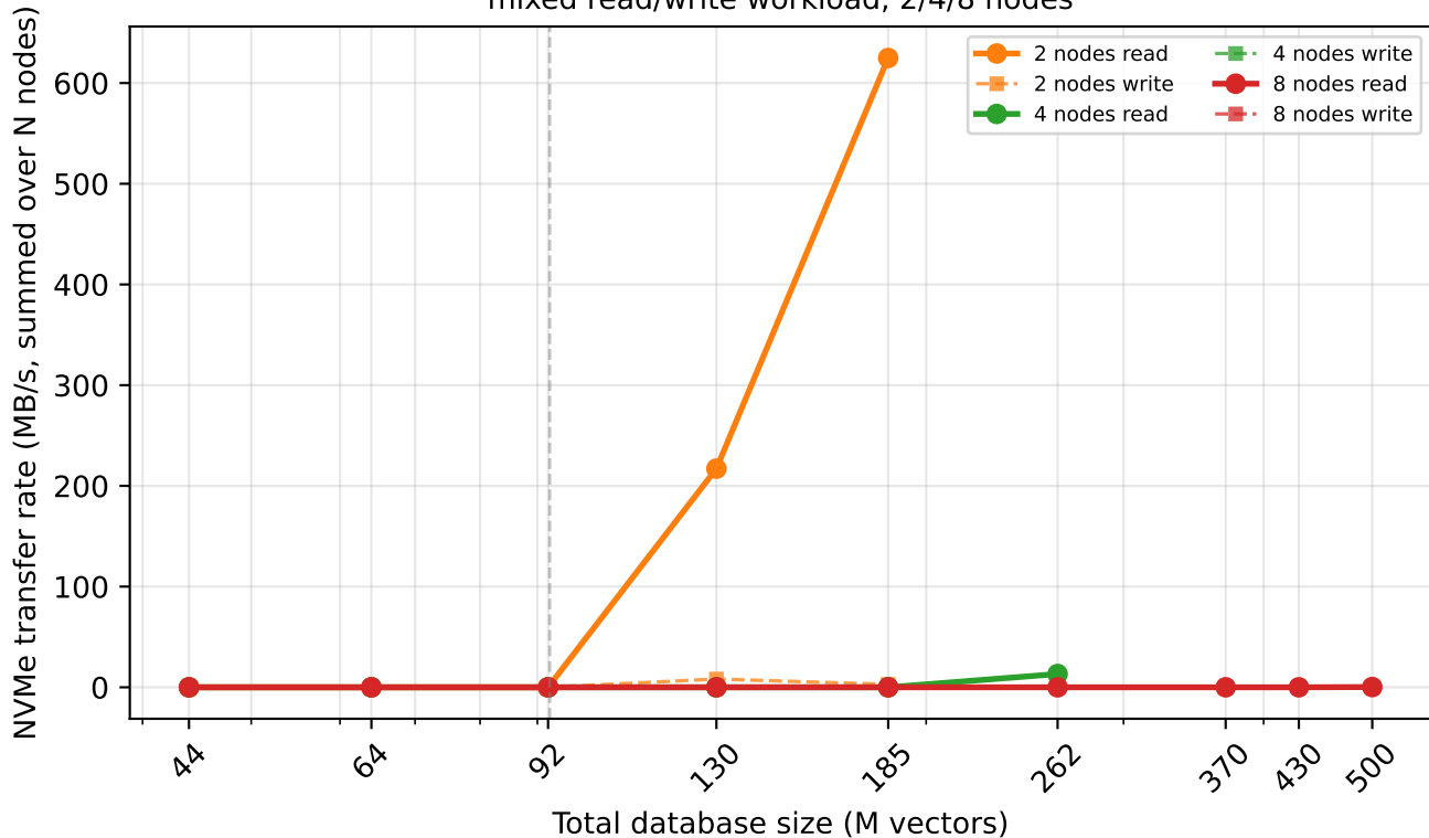
Aggregate NVMe transfer rate vs. database size mixed read/write workload, 2/4/8 nodes
