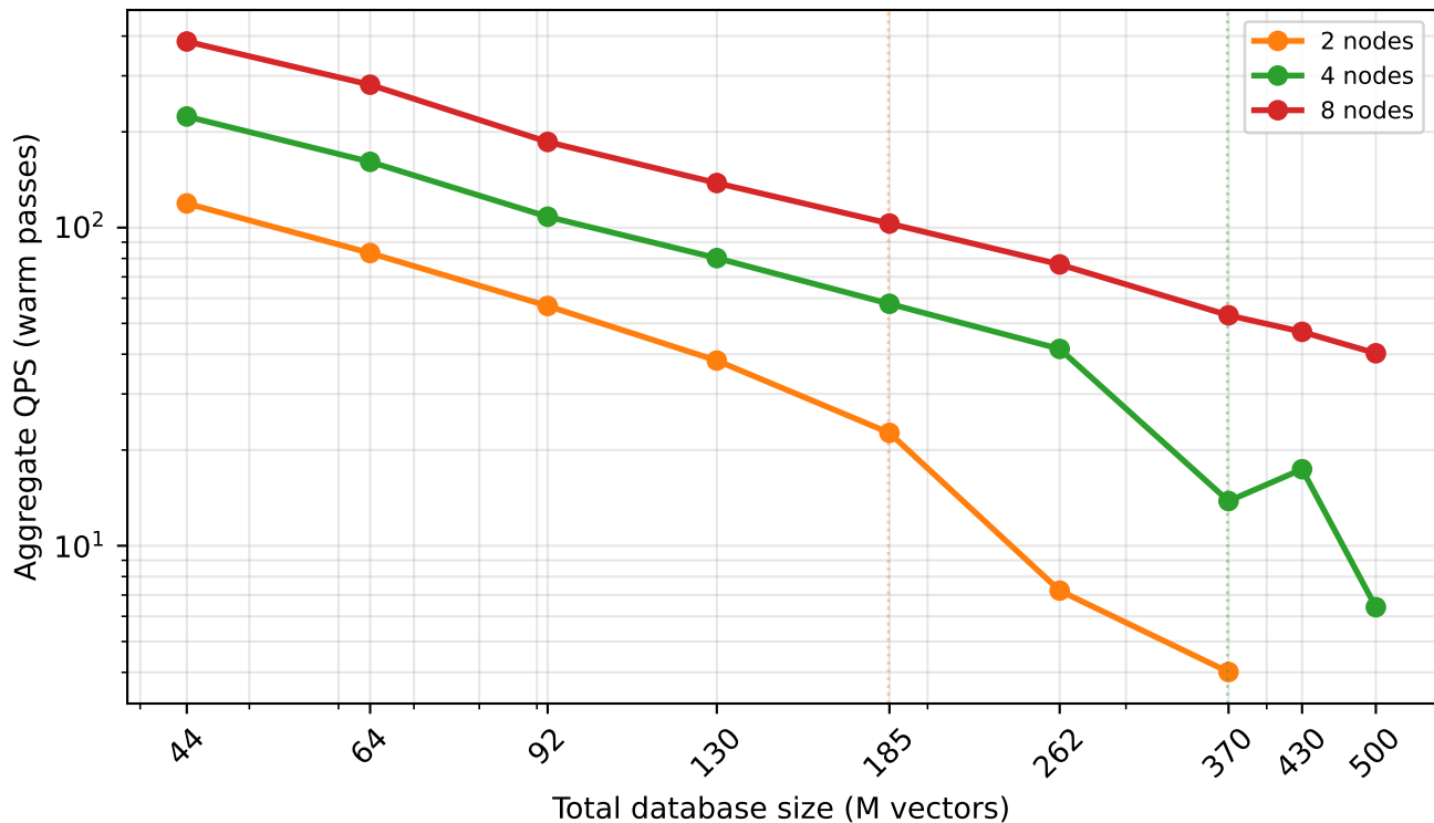
Read-only search throughput 2/4/8 nodes (dotted lines: per-node RAM limit \times node count)
