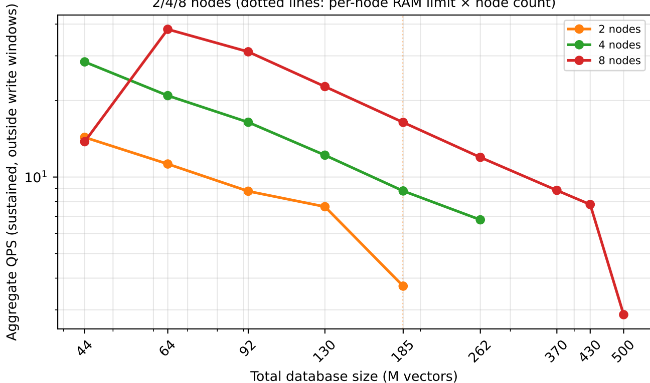
Search throughput under a mixed read/write workload 2/4/8 nodes (dotted lines: per-node RAM limit \times node count)
