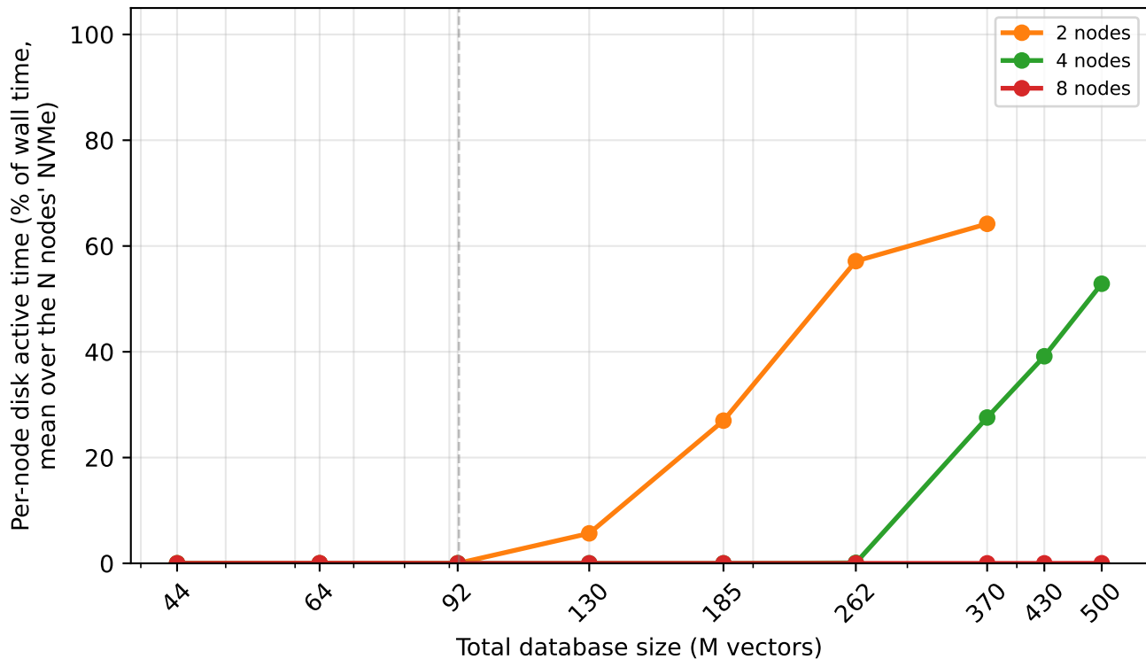
Per-node NVMe active time vs. database size read-only workload, 2/4/8 nodes
