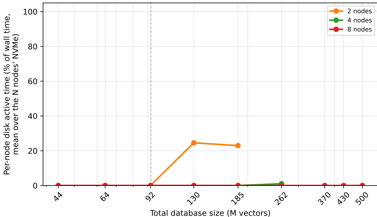
Per-node NVMe active time vs. database size mixed read/write workload, 2/4/8 nodes
