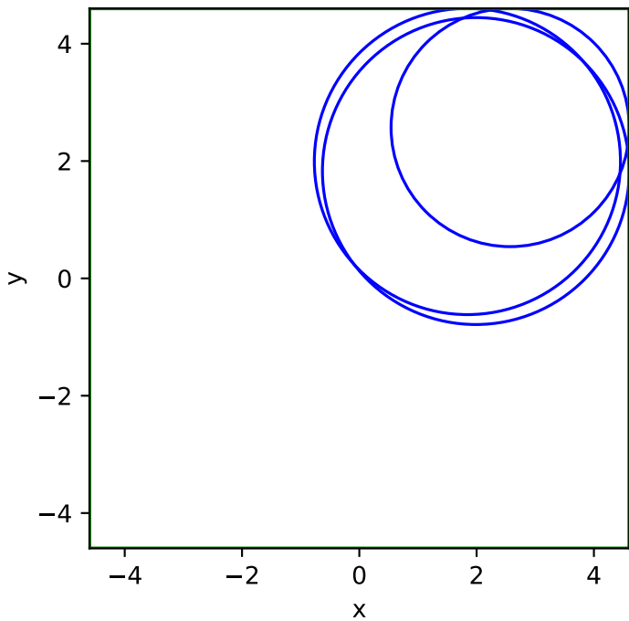
Circle packing (ratio=0.659)
