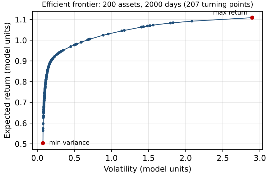
Figure 1: The efficient frontier of the 200-asset, 2000-day problem in expected-return / volatility space, computed exactly by the Critical Line Algorithm. Each marker is one of the 207 turning points; the endpoints are the maximum-return portfolio ( \lambda = \infty ) and the global minimum-variance portfolio ( \lambda = 0 ).
