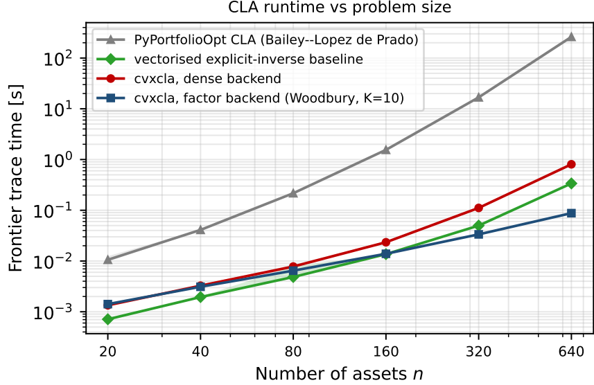
Figure 2: Frontier trace time as a function of the number of assets n (log–log). PyPortfolioOpt (Martin, 2021), a critical-line implementation in pure Python, scales like \approx n^{3.4} ; the vectorised explicit-inverse baseline of §9.3 like \approx n^{2.0} ; cvxcla’s dense backend like \approx n^{2.2} ; and its diagonal-plus-low-rank factor backend, solving the identical covariance through the Woodbury identity, like \approx n^{1.3} . At n = 640 the factor backend is roughly 2980\times faster than PyPortfolioOpt and 9\times faster than the dense backend. The incremental-inverse baseline and the dense backend lie close together, far below PyPortfolioOpt. Markers are the median of 3 repetitions; the shaded band around each spans their min and max.
