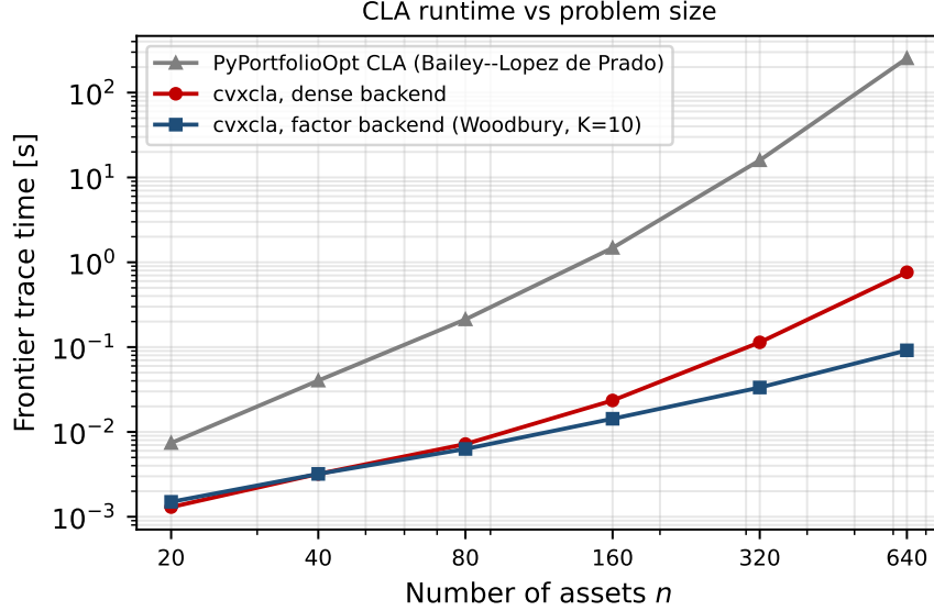
Figure 2: Frontier trace time as a function of the number of assets n (log–log). PyPortfolioOpt (Martin, 2021), a critical-line implementation in pure Python, scales like \approx n^{3.4} ; cvxcla ’s dense backend like \approx n^{2.2} ; and its diagonal-plus-low-rank factor backend, solving the identical covariance through the Woodbury identity, like \approx n^{1.3} . At n = 640 the factor backend is roughly 2800\times faster than PyPortfolioOpt and 8\times faster than the dense backend.
