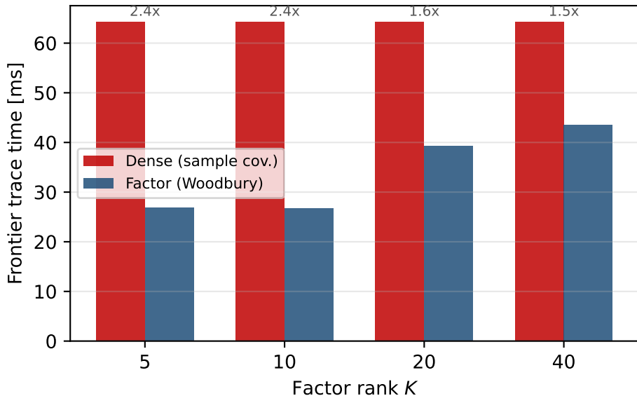
Dense vs factor backend on S\&P 500 ( N = 494 assets)
