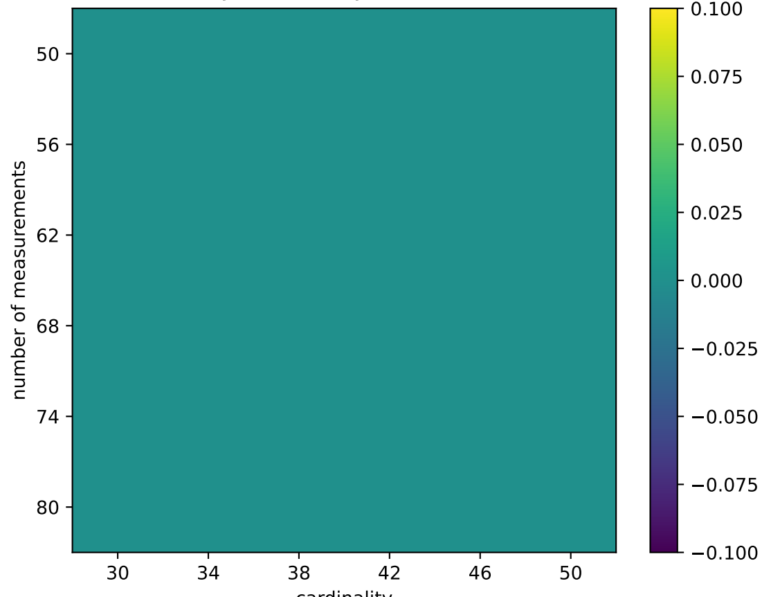
Probability of recovery: \ell_1 norm (convex)
