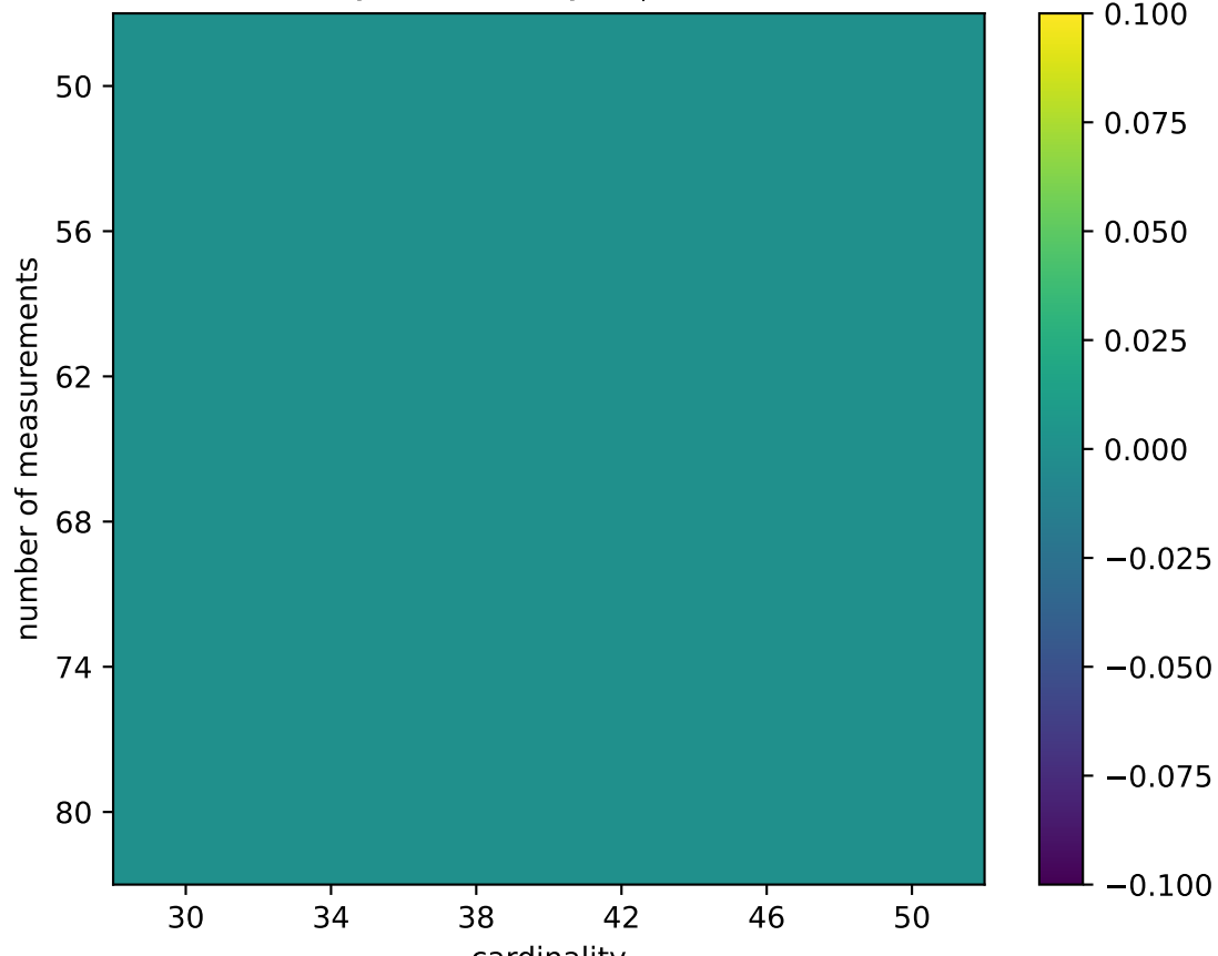
Probability of recovery: \ell_{1/2} norm (DCCP)
