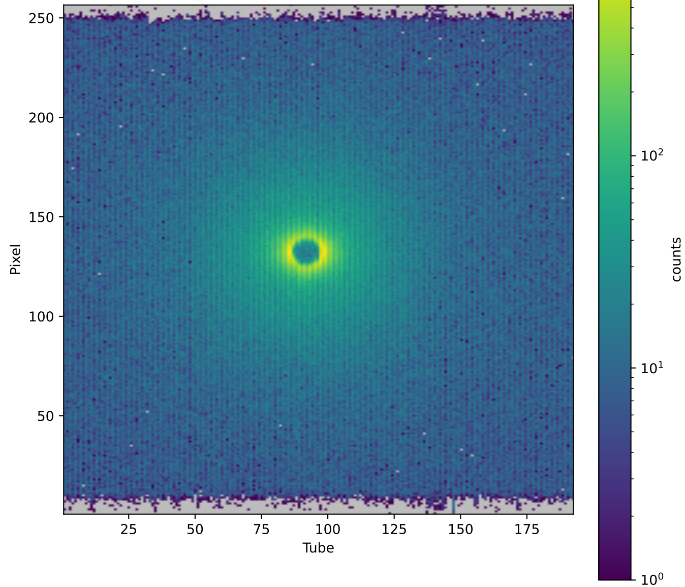
EQSANS_172749 — S-sam9 SR-0.001 4m10a sa6mm
