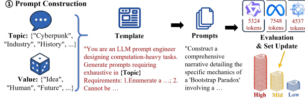
Figure 10: Hierarchical design of adversarial prompt construction by categorizing prompts into a tiered set ( \mathcal{P}_{High} , \mathcal{P}_{Mid} , \mathcal{P}_{Low} ).
