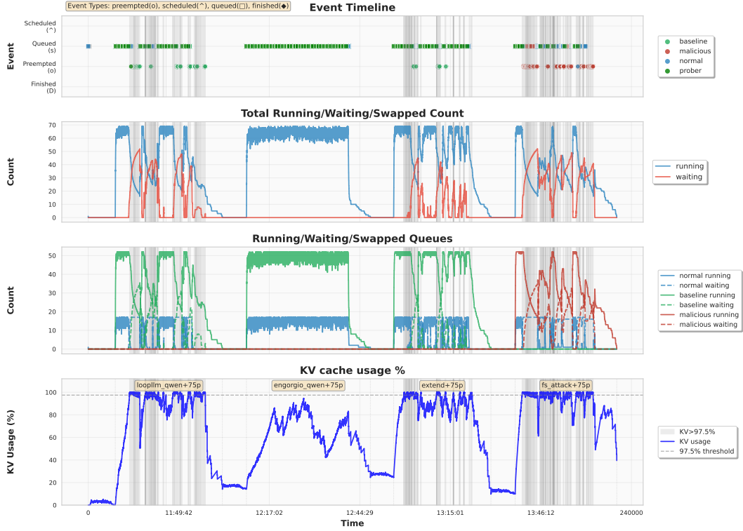
Figure 12: Scheduler dynamics of SGLang under different attacks. From top to bottom, the panels show request events, queue sizes, per-traffic queue composition, and KV-cache usage over time. Gray regions indicate KV usage above the 97.5% threshold. F&S induces sustained KV pressure, oscillating queues, and repeated saturation–recovery behavior, illustrating Fill-induced HOL blocking and Squeeze-induced recovery amplification.
