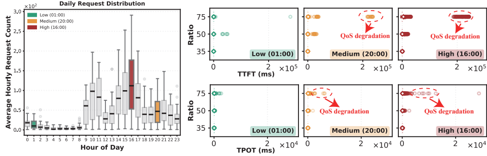
Figure 7: Attack impact on normal users under real-world traffic patterns. Left: Hourly request distribution from BurstGPT traces with three representative traffic intensities. Right: TTFT and TPOT distributions for normal users under varying malicious ratios.
