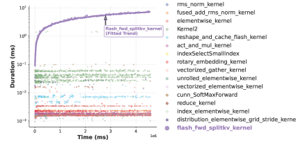
Figure 2: CUDA kernel execution under the latency attack.
