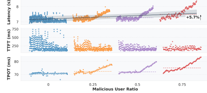
Figure 1: Impact of latency attacks on normal users.
