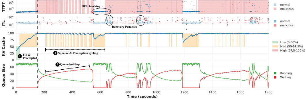
Figure 5: Visualization of TTFT, ITL, Global KV-Cache usage and queue size of F&S attack over time. The Waiting Queue Size (bottom) accumulates as opposed to the Running Queue, which directly correlates with the massive outliers observed in the TTFT Scatter Plot (top right), where user requests are blocked for tens of seconds before processing begins, confirming that the TTFT surge stems from HOL blocking.
