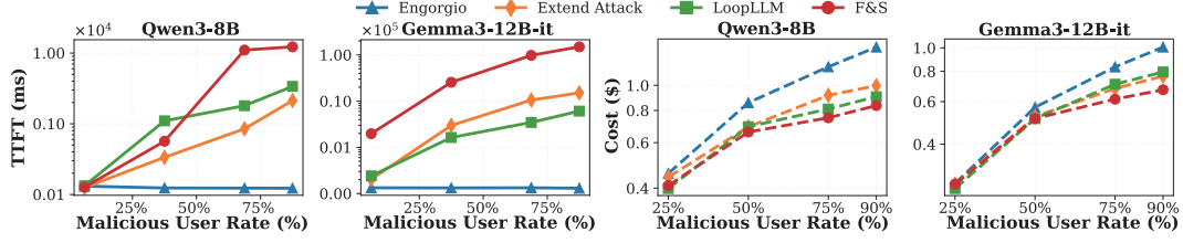
Figure 6: Impact of malicious user rate on attack efficacy and cost across different model architectures.
