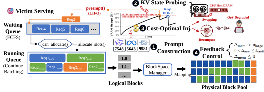
Figure 3: Overview of F&S attack steps and scheduling states, in which a key is the transition between the FCFS-based Waiting Queue and the continuously-batched Running Queue.
