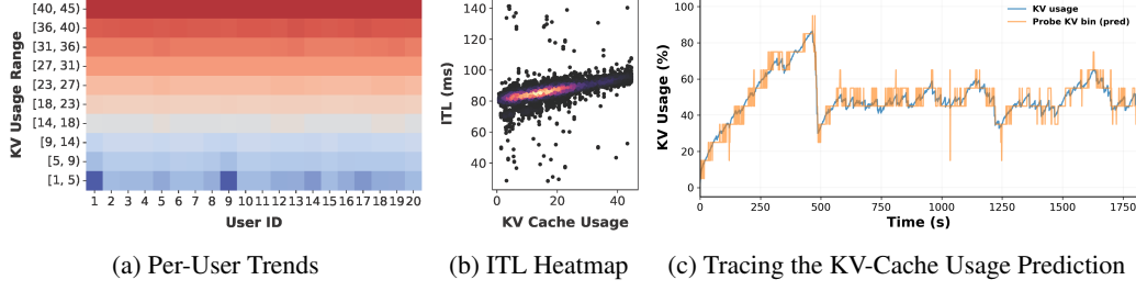
Figure 4: Black-box estimation of KV usage on Qwen3-8B. (a) Similar latency imposed on all users due to shared memory contention; (b) strong linear correlation between ITL and global KV-cache usage ( U_{\text{sys}} ); (c) trace of KV-cache estimation accuracy using LightGBM.
