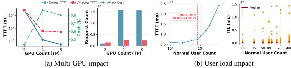
Figure 8: Multi-GPU scalability analysis under varying hardware resources and load configurations.
