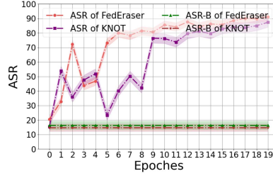
(b) CIFAR-10
