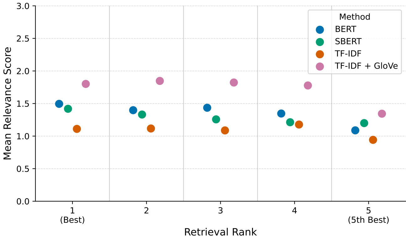
Mean Relevance Score by Retrieval Rank and Method
