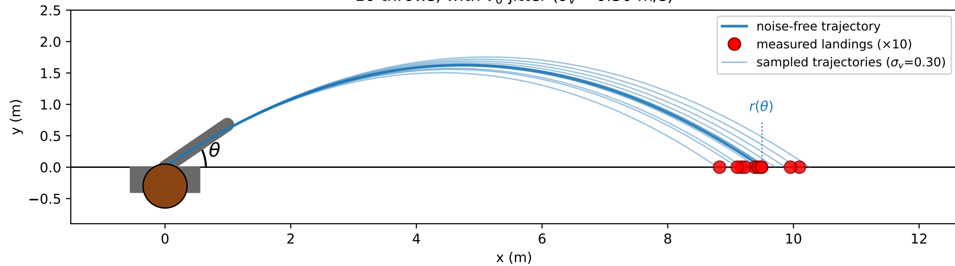
10 throws, with v_0 jitter ( \sigma_v = 0.30 m/s)
