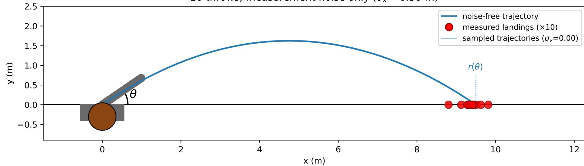
10 throws, measurement noise only ( \sigma_x = 0.30 m)
