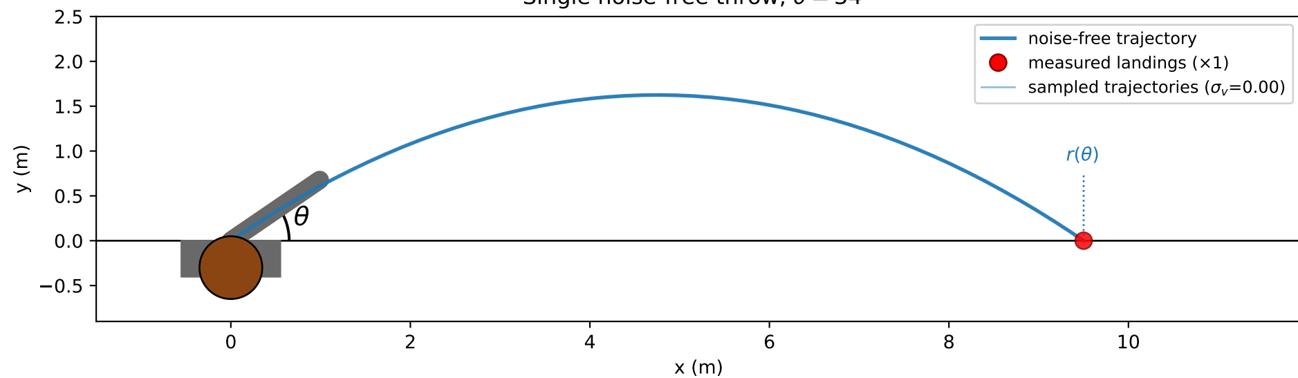
Single noise-free throw, \theta = 34^\circ
