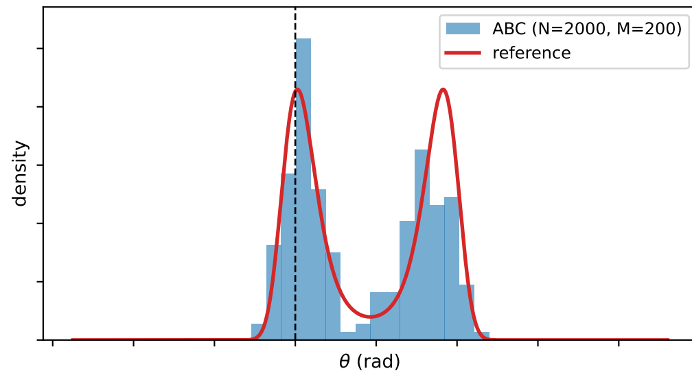
N=2000, M=200 (cleaner)
