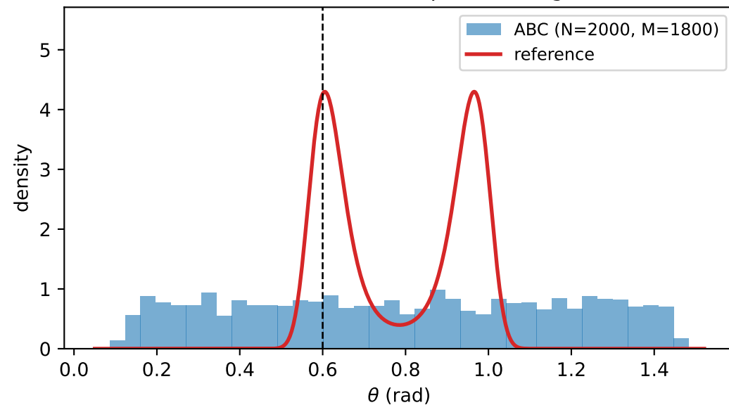
N=2000, M=1800 (prior leakage)
