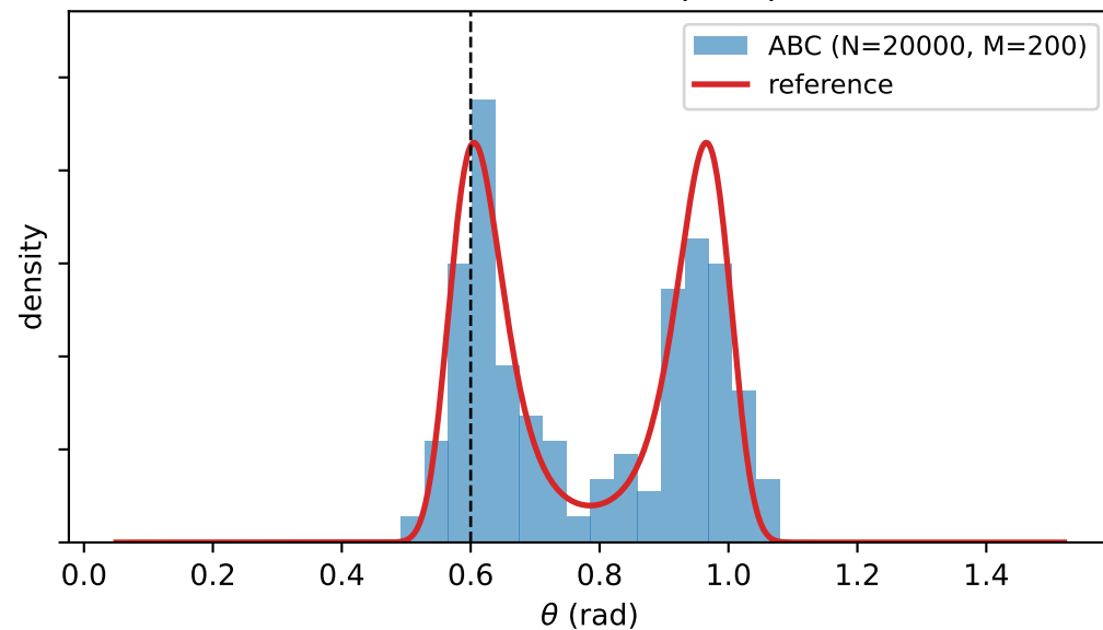
N=20000, M=200 (sharp, expensive)
