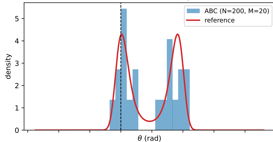
N=200, M=20 (noisy)
