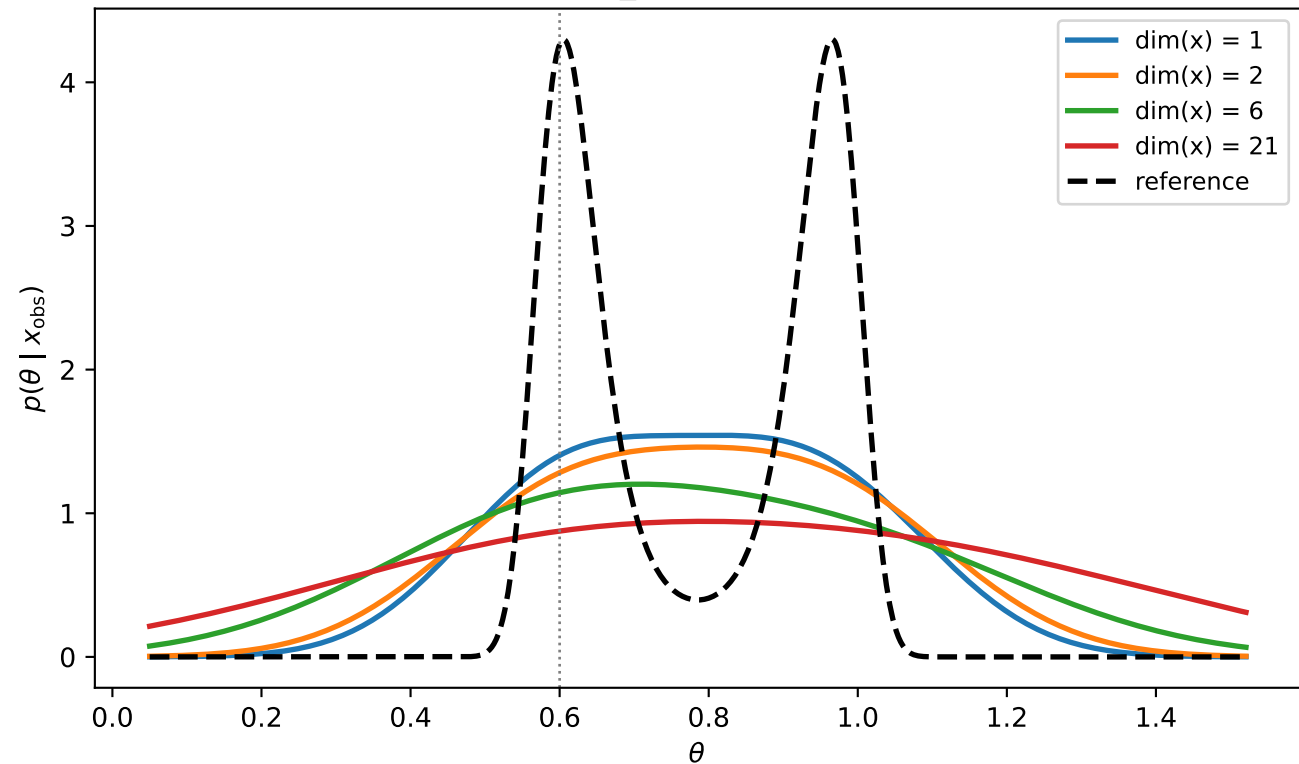
KDE posterior as we pad x_{\text{obs}} with uninformative dimensions
