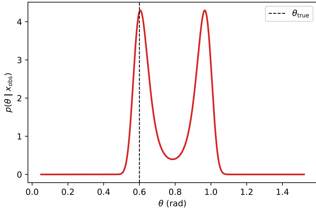
Reference posterior at x_{\text{obs}} = 9.54
