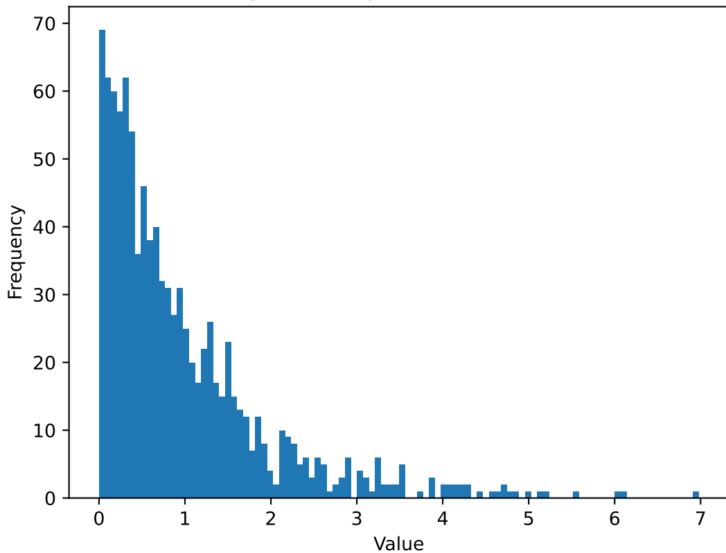
Histogram of Exponential Distribution
