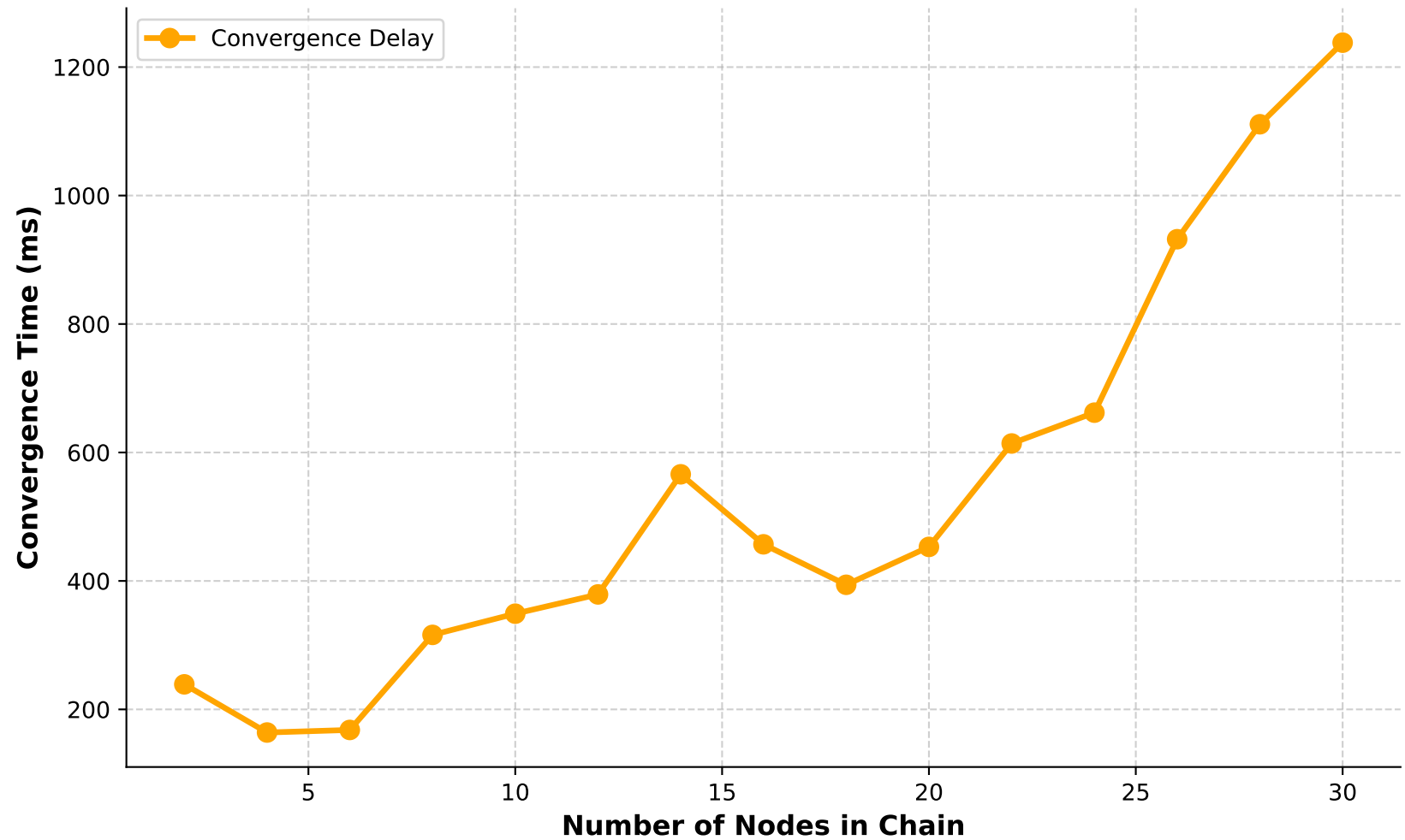
Total Convergence Time vs Linear Chain Size
