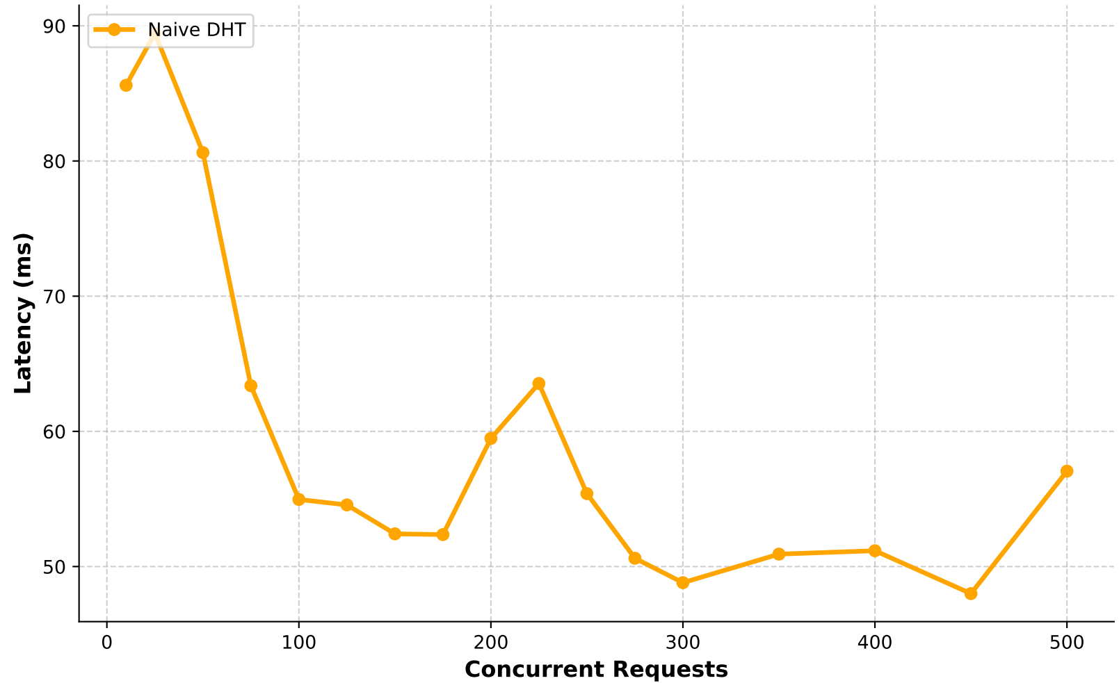
Average Request Latency vs Load
