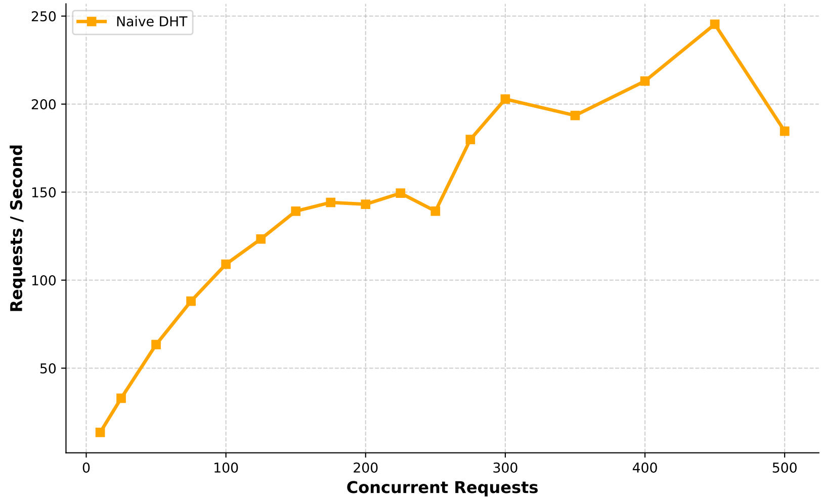
Global System Throughput vs Load
