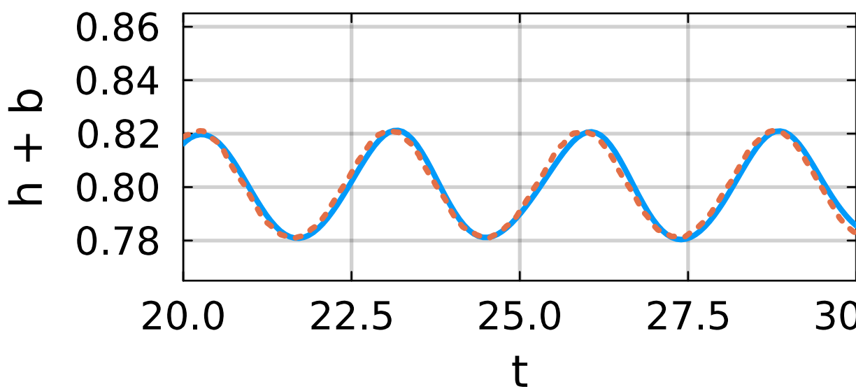
Gauge at x = 3.04
