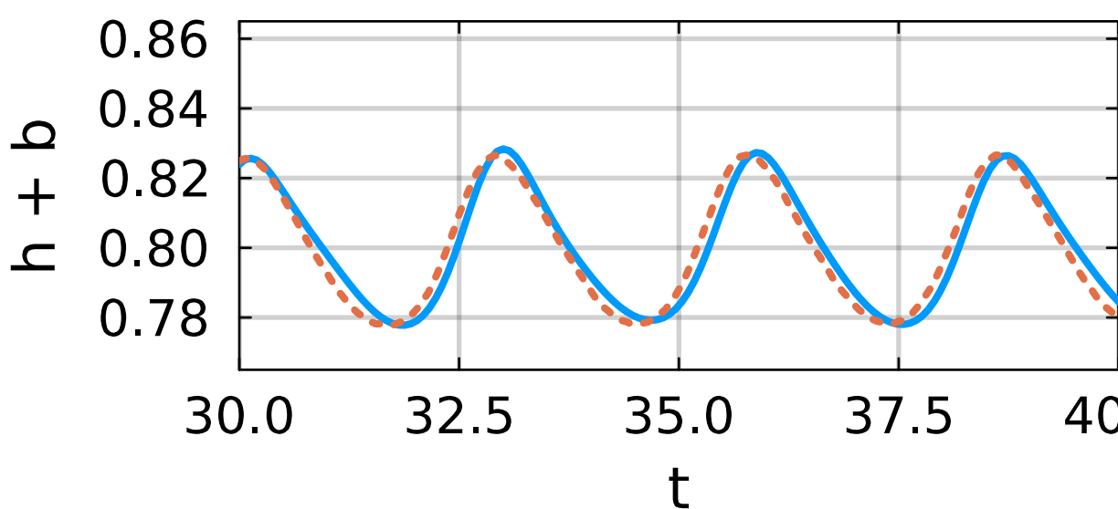
Gauge at x = 20.04
