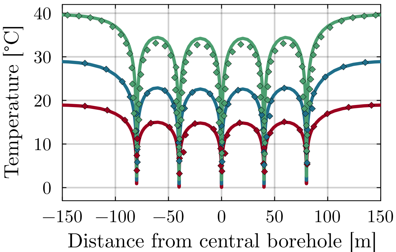
Array Spacing of 40 m
