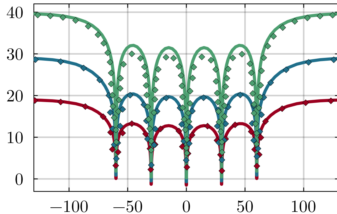
Array Spacing of 50 m
