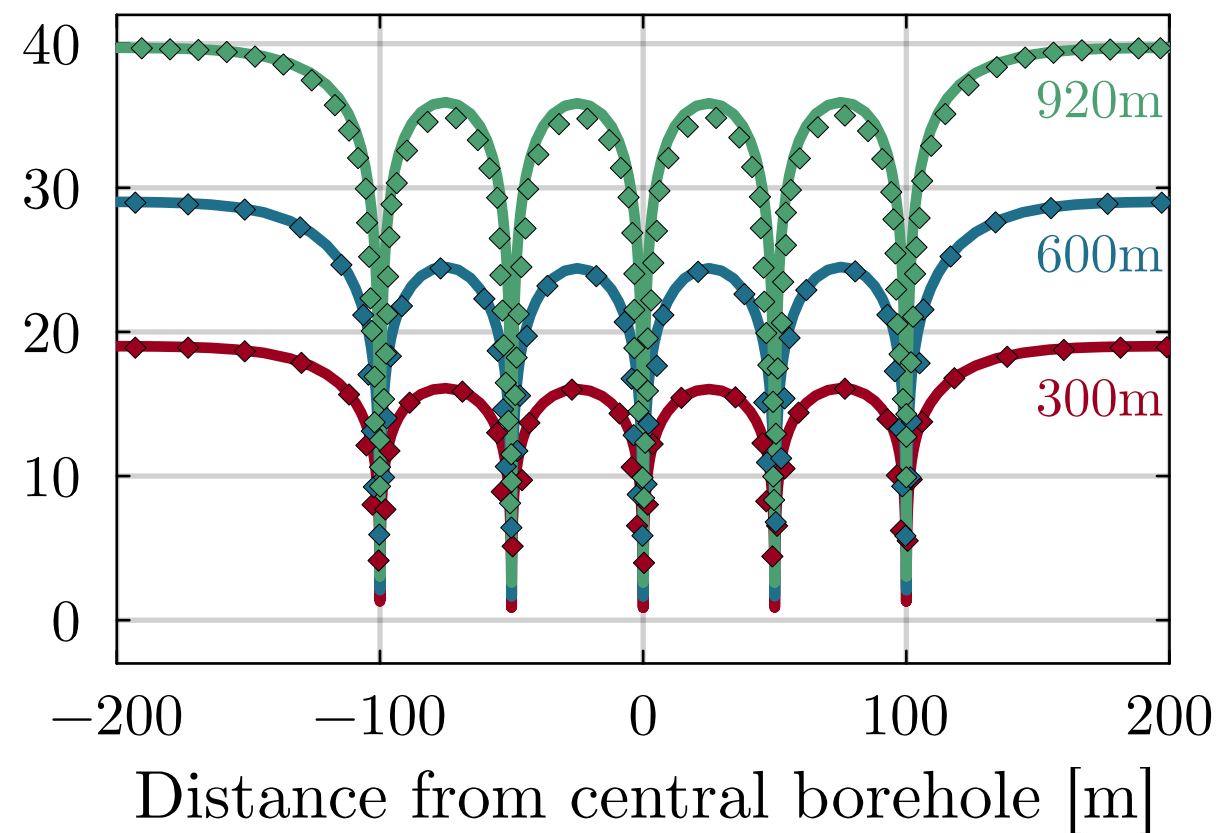
Array Spacing of 50 m
