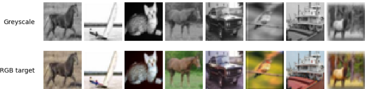
Figure 1: Each column pairs a greyscale training image with the RGB target we want the network to predict. To plot the two rows together, expand repeats each grey value across RGB, while the network itself still receives just one channel.
