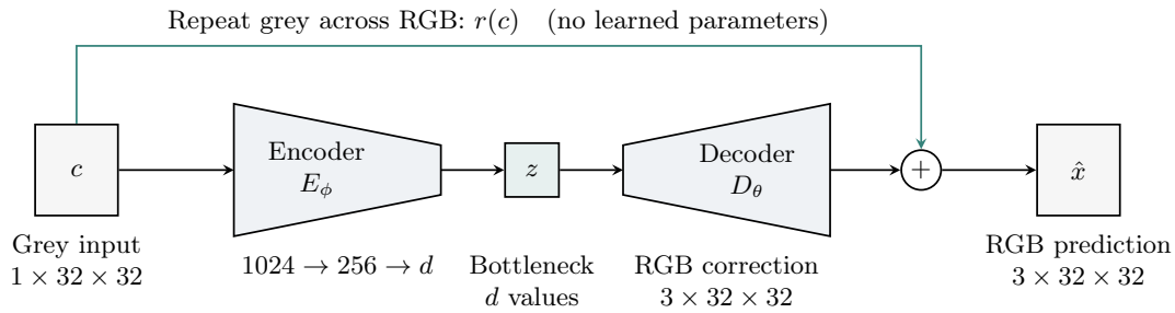
Figure 3: A fixed skip connection carries the grey pixels around the bottleneck. The decoder now predicts a correction, which is added pixel by pixel to the repeated-grey image. Unlike the U-Net in Lecture 3, this model has a single image-to-output skip, without connections between intermediate feature layers.
