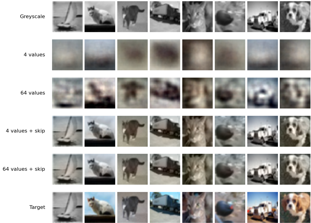
Figure 4: The first eight validation images. Four latent values retain broad regions of light and colour; 64 retain more structure. With a skip, image detail can bypass either bottleneck. Each model uses 6,000 updates.
