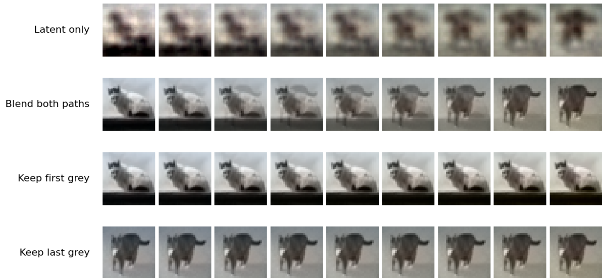
Figure 5: Left to right: a = 0 to a = 1 . The top row uses the plain 64-value MLP. The remaining rows use the 64-value skip model with different inputs on its grey path.
