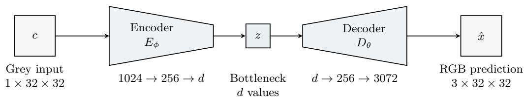
Figure 2: An encoder–decoder for colourisation, with image shapes written as channels \times height \times width (omitting the batch dimension). Layer widths appear below each network, and both use a ReLU after the hidden layer of width 256. As in Lecture 3’s autoencoder, the input is compressed into a vector and then expanded into an image, but here the target is RGB and the input is grey.
