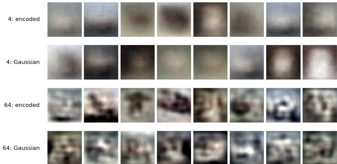
Figure 7: Predictions from encoded validation images, followed by Gaussian latent samples. The sampled rows have no paired target image. Four values produce smooth regions resembling the severely compressed reconstructions; the 64-value decoder can also produce more complicated, implausible arrangements.
