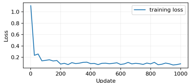
Figure 1: First fixed sample batch and training losses from this run. Running the program creates all sample files.
