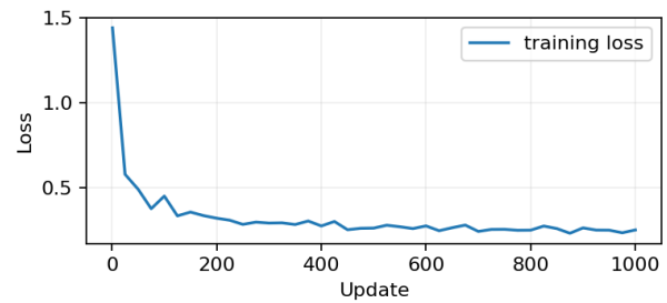
Figure 2: First fixed sample batch and training losses from this run. Running the program creates all sample files.
