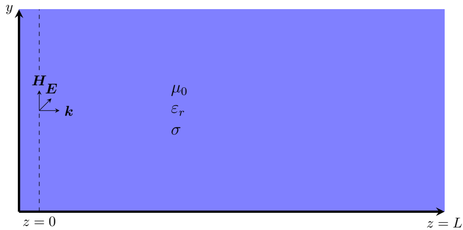
Figure 2: Uniform plane wave geometry.
