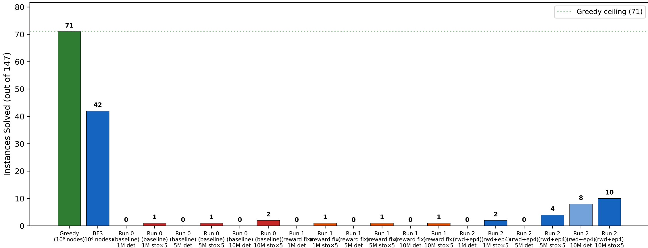
Mini Experiment: Solve Counts by Algorithm and Checkpoint
