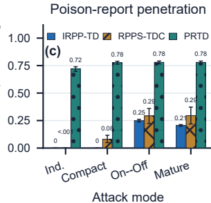
Malicious-report leakage
