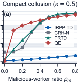
Active-task NRMSE
