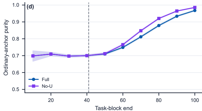
Uncertainty ablation under delayed poisoning
