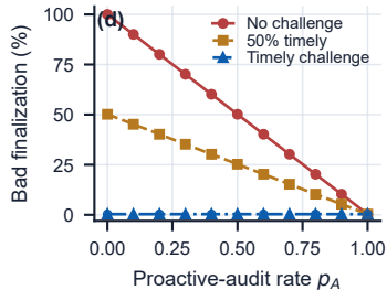
Conditional accountability
