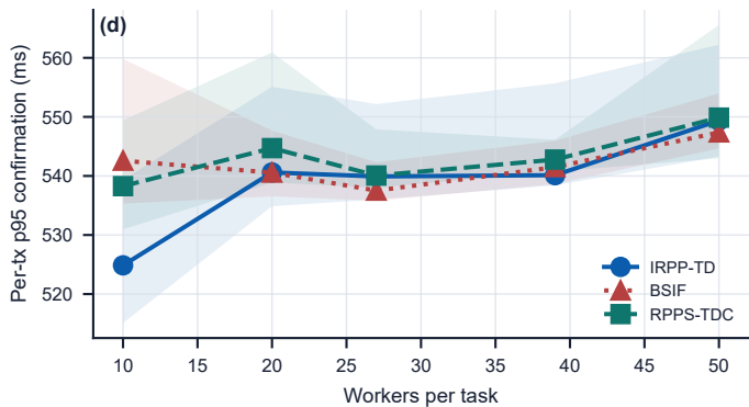
Consensus confirmation
