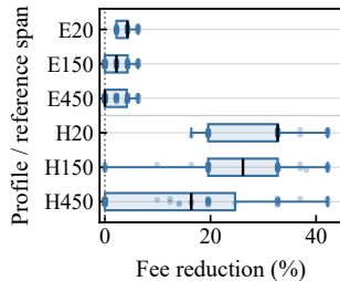
(a) Versus JB-RobustD
