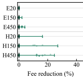
(b) Versus Greedy
