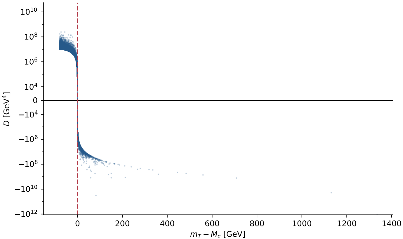
Fixed mass 80.3625 GeV: all 100,000 events
