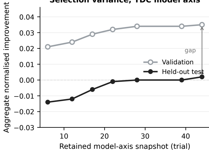
Selection variance, TDC model axis
