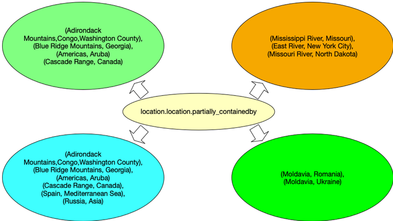
Fig. 6. Multiple types of entities of relation location (the relation HasPart has at least two latent semantics: composition related as (Table, HasPart, Leg) and location related as (Atlantic, HasPart, NewYorkBay) ) (Ji et al., 2015) .
