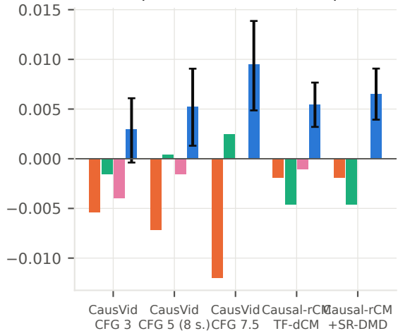
A5 temporal coherence (-warp error)
