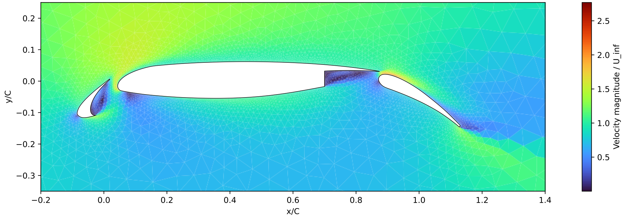
Actual Gmsh cell field: UNCONVERGED; accuracy NOT accepted
