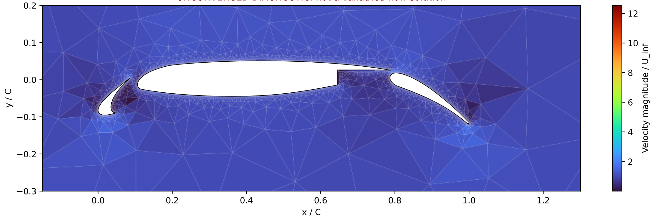
30P30N: Velocity magnitude / U_{\infty} UNCONVERGED DIAGNOSTIC: not a validated flow solution
