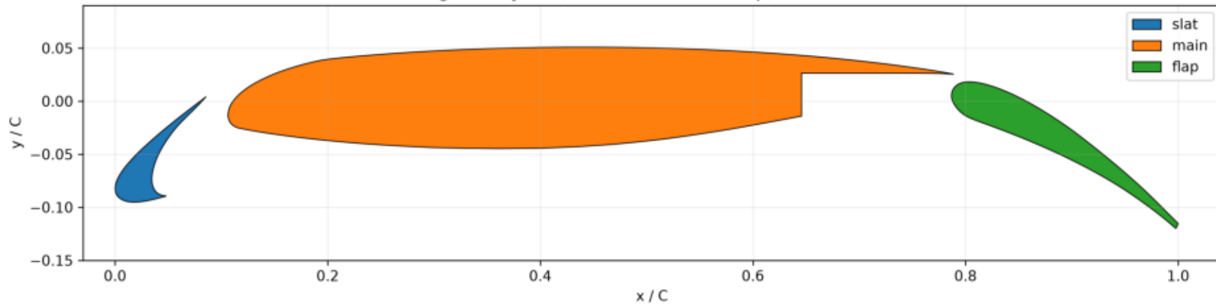
30P30N geometry: slat, main element and flap; fluid slots retained
