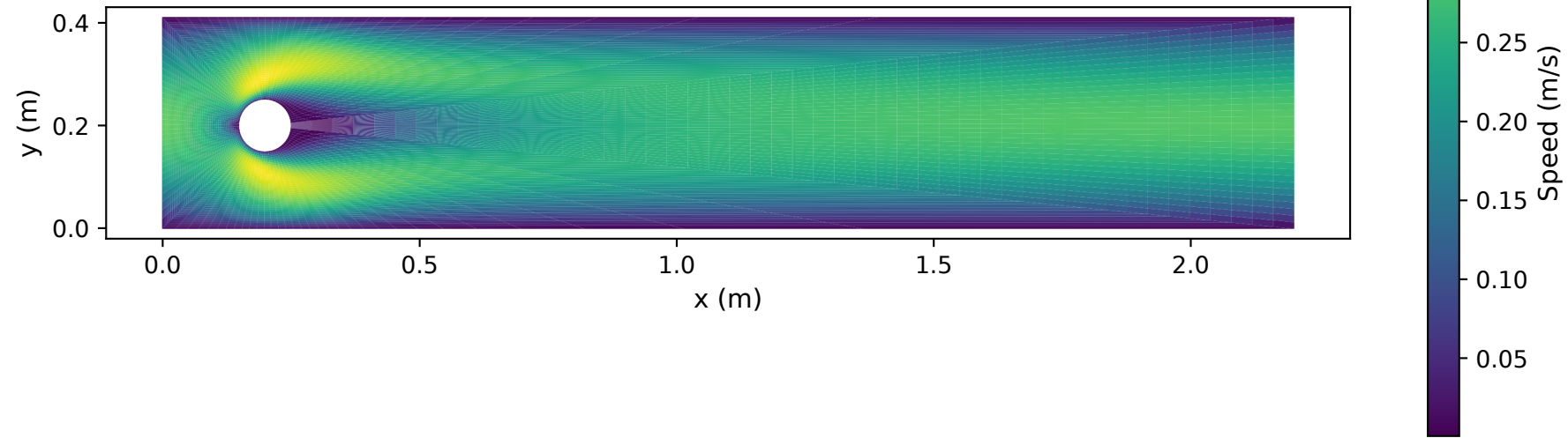
cylinder 128x48
