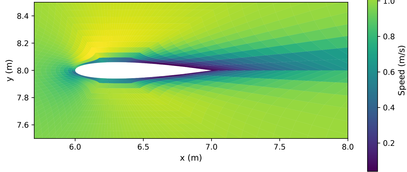
Wall and wake detail: 128x52
