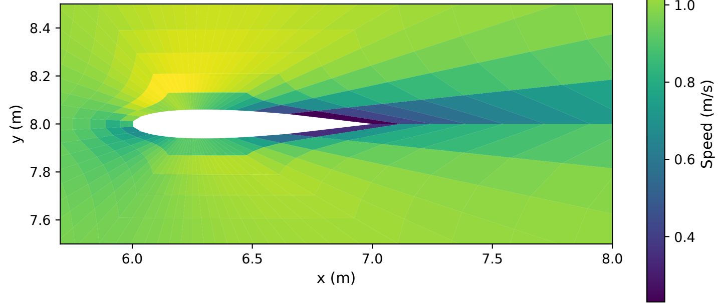
Wall and wake detail: 64x26
