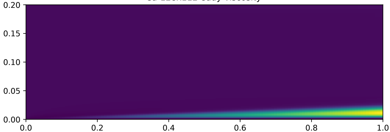
sa-128x112 eddy-viscosity
